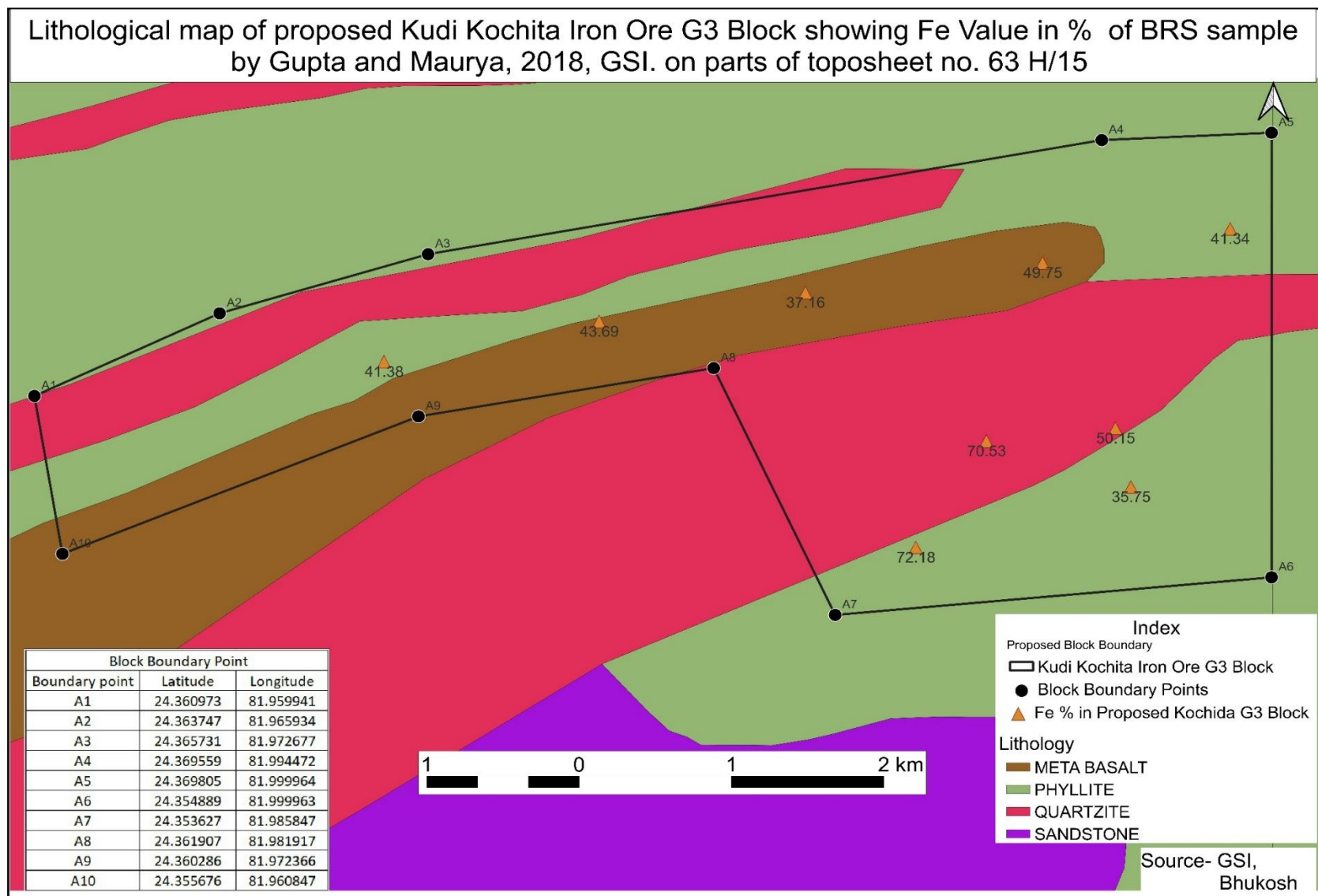
Plate 4: Block boundary over geological map showing distribution of Fe 2 O 3 % in BRS over proposed Block boundary area.
